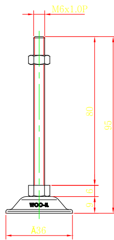
BL36-M6-80
