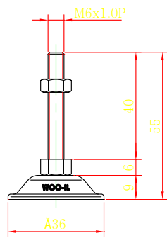
BL36-M6-40
