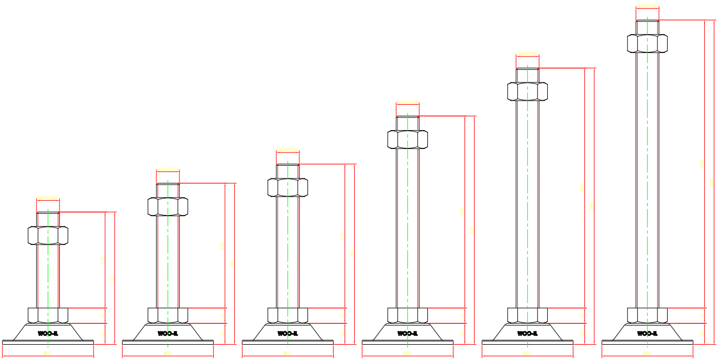
BL95-M24-100
