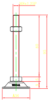
BL36-M8-80
