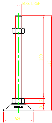
BL36-M8-100
