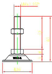
BL36-M8-40
